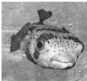
Alpha blending
