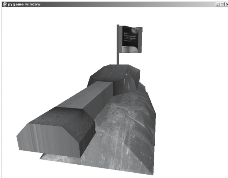
Figure 11-6. tankdemo.py
