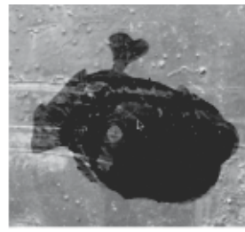
Subtractive blending
