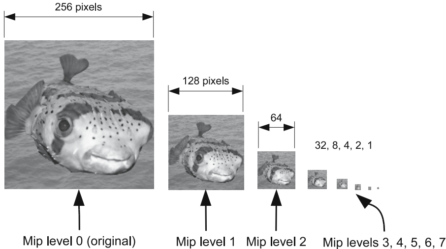
Figure 11-3. Mip maps
