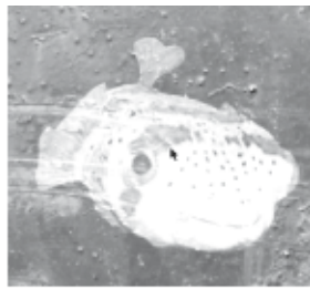
Additive blending
